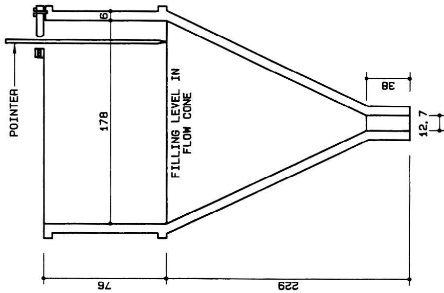
FLOW CONE
